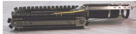
RST 8" Crawler
